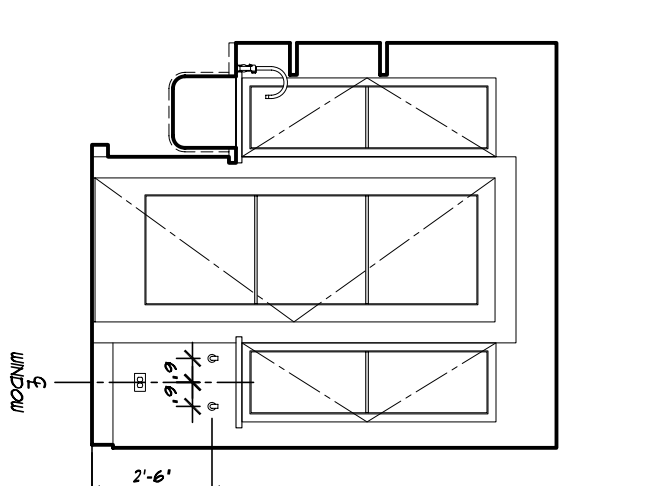
17 LAUNDRY SOUTH A5.3 1/4" = 1'-0"
