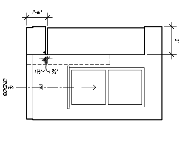
19 MUD ROOM NORTH A5.3 1/4" = 1'-0"
