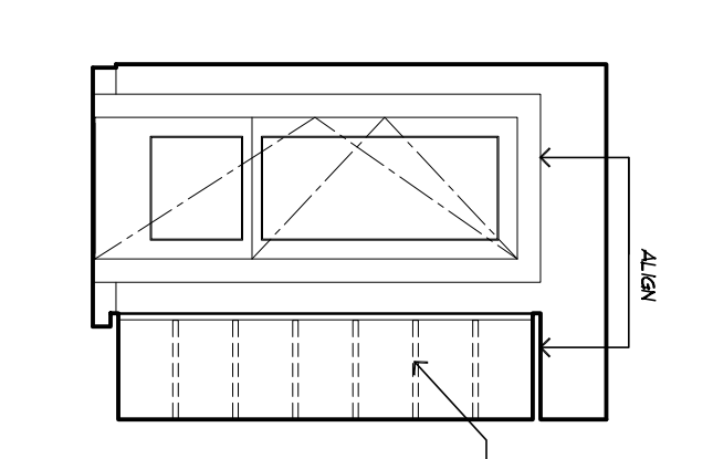
21 MUD ROOM SOUTH A5.3 1/4" = 1'-0"
